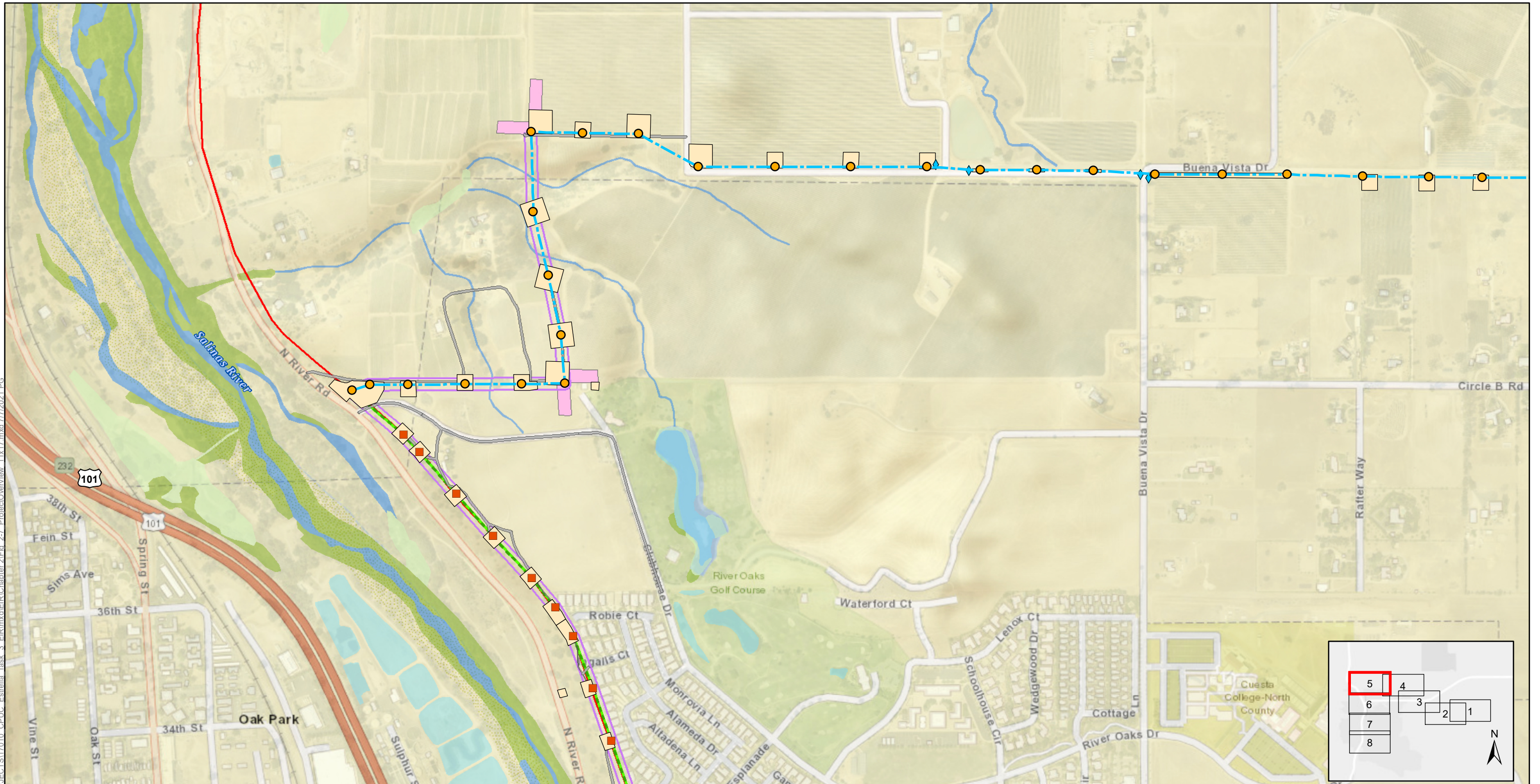
Figure 2-7 Estrella Substation and 70 kV Power Line Components - Detailed View Sheet 5 of 8
